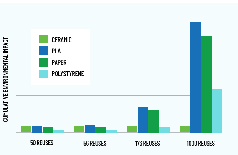
Fig 5. Cumulative environmental impact of ceramic plate vs. various disposable options over time.
